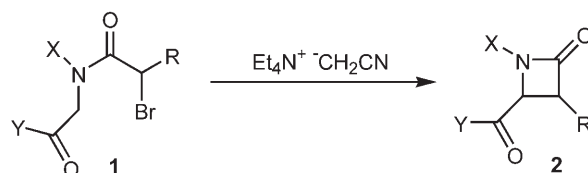
Scheme 3. General reaction Scheme for the electrochemically induced synthesis of \beta -lactams.
