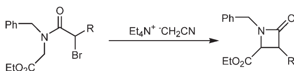
Scheme 2. Electrochemically induced synthesis of \beta -lactams by C-3–C-4 bond formation.
